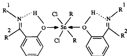
26 a R, R^1 = \text{CH}_3, \text{C}_2\text{H}_5, \text{C}_4\text{H}_9; R^2 = \text{H}
